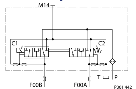
EDC-Schematic diagram
